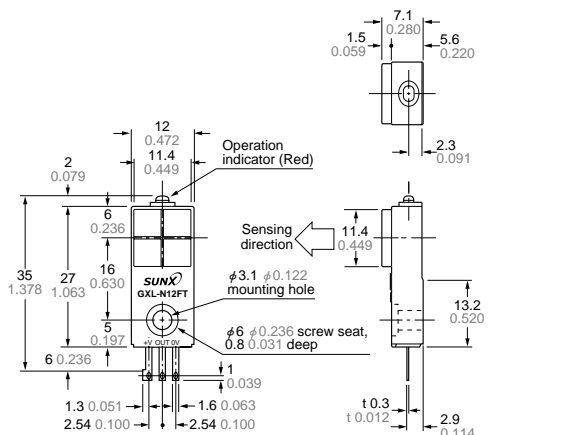
GXL-N12FT type Sensor
